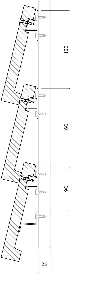
Vertical cut 1:5
