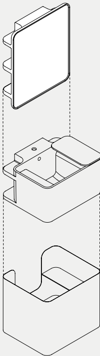
70,5×60 cm ANF-SP Specchio portaoggetti in ceramica. Ceramic mirror with storage.
