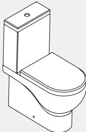
65×35×H84 cm NUVCMP000000 Vaso monoblocco filomuro. Wall trap close coupled wc.
