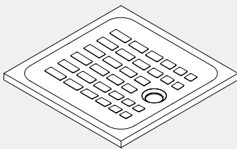
90×90×H4 cm CBPD09009040 Piatto doccia Puro quadrato 90×90 cm. 90×90 cm squared shower tray.
